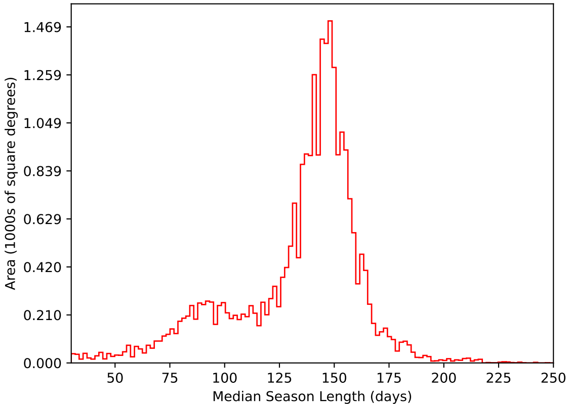
ddf_loaded_fl4_v3.4_10yrs All sky i band: Median Season Length
