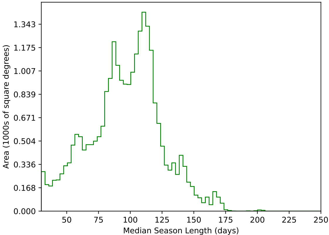
ddf_loaded_fl4_v3.4_10yrs All sky g band: Median Season Length
