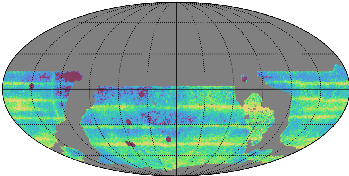
ddf_loaded_fl4_v3.4_10yrs WFD: Median Intra-Night Gap
