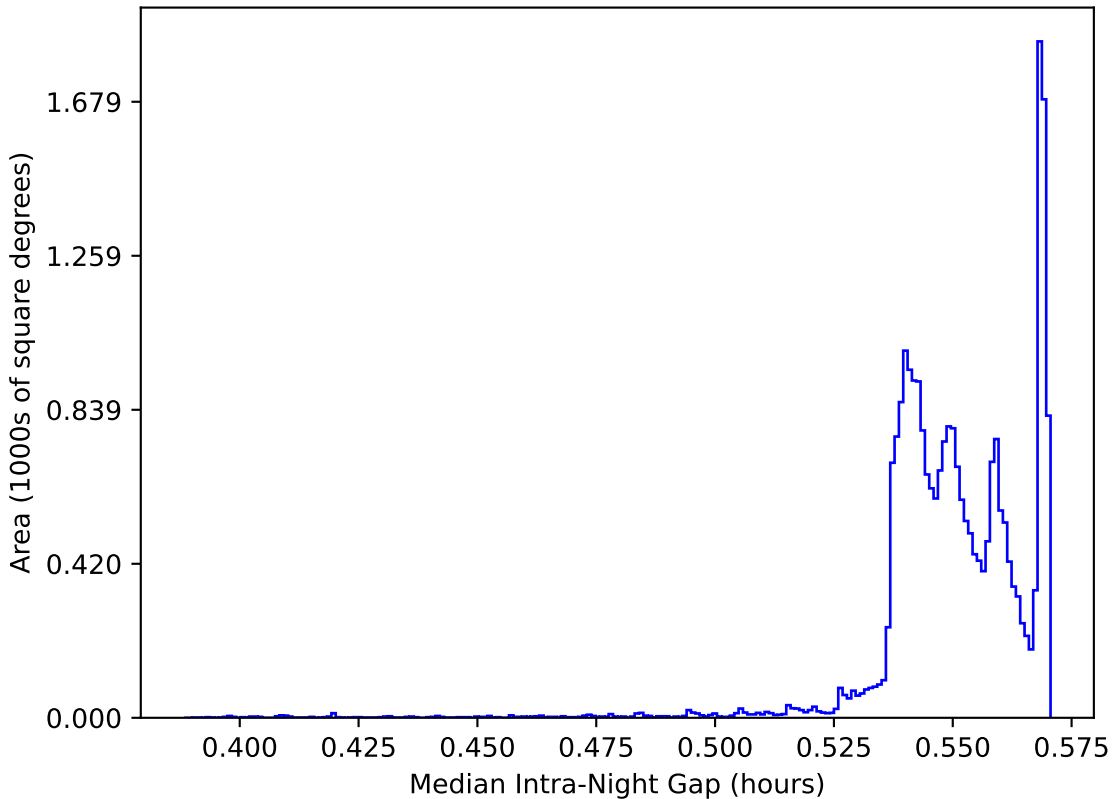
ddf_loaded_fl4_v3.4_10yrs All sky: Median Intra-Night Gap
