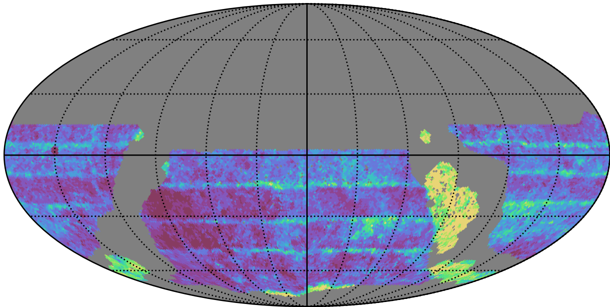
ddf_loaded_fl4_v3.4_10yrs WFD z band: Median Inter-Night Gap
