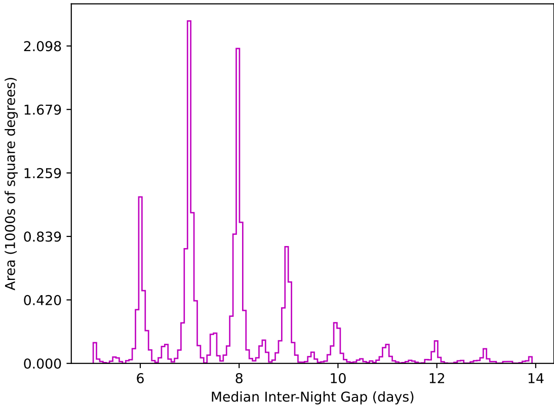
ddf_loaded_fl4_v3.4_10yrs WFD z band: Median Inter-Night Gap
