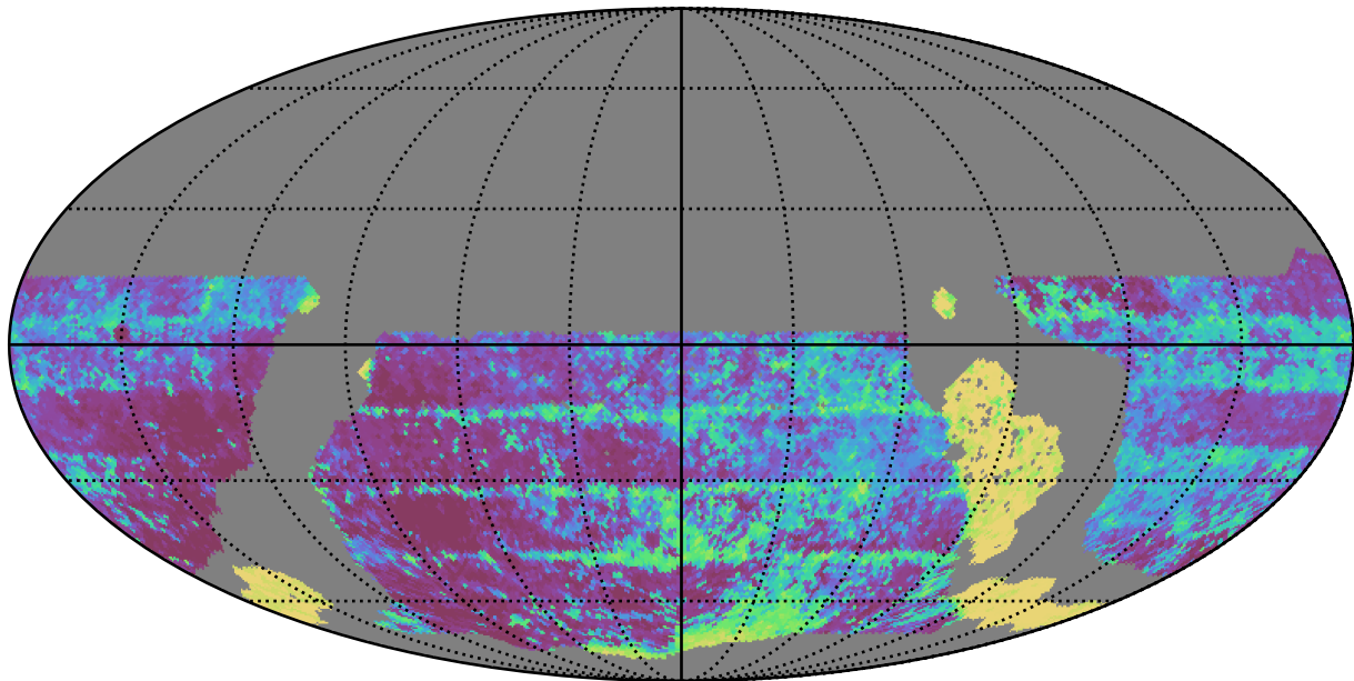
ddf_loaded_fl4_v3.4_10yrs WFD y band: Median Inter-Night Gap
