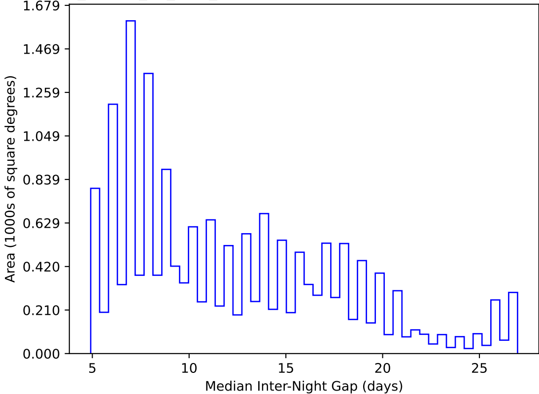
ddf_loaded_fl4_v3.4_10yrs WFD y band: Median Inter-Night Gap
