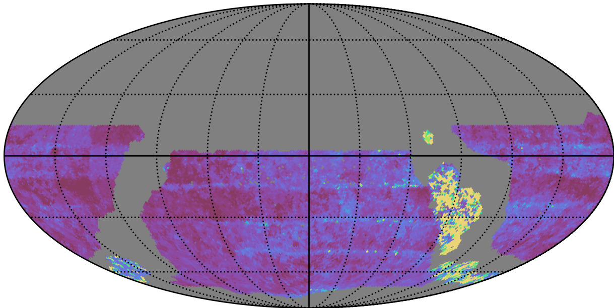
ddf_loaded_fl4_v3.4_10yrs WFD u band: Median Inter-Night Gap
