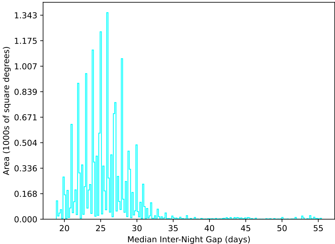
ddf_loaded_fl4_v3.4_10yrs WFD u band: Median Inter-Night Gap
