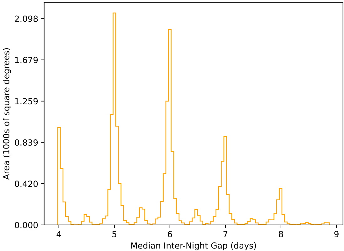
ddf_loaded_fl4_v3.4_10yrs WFD r band: Median Inter-Night Gap
