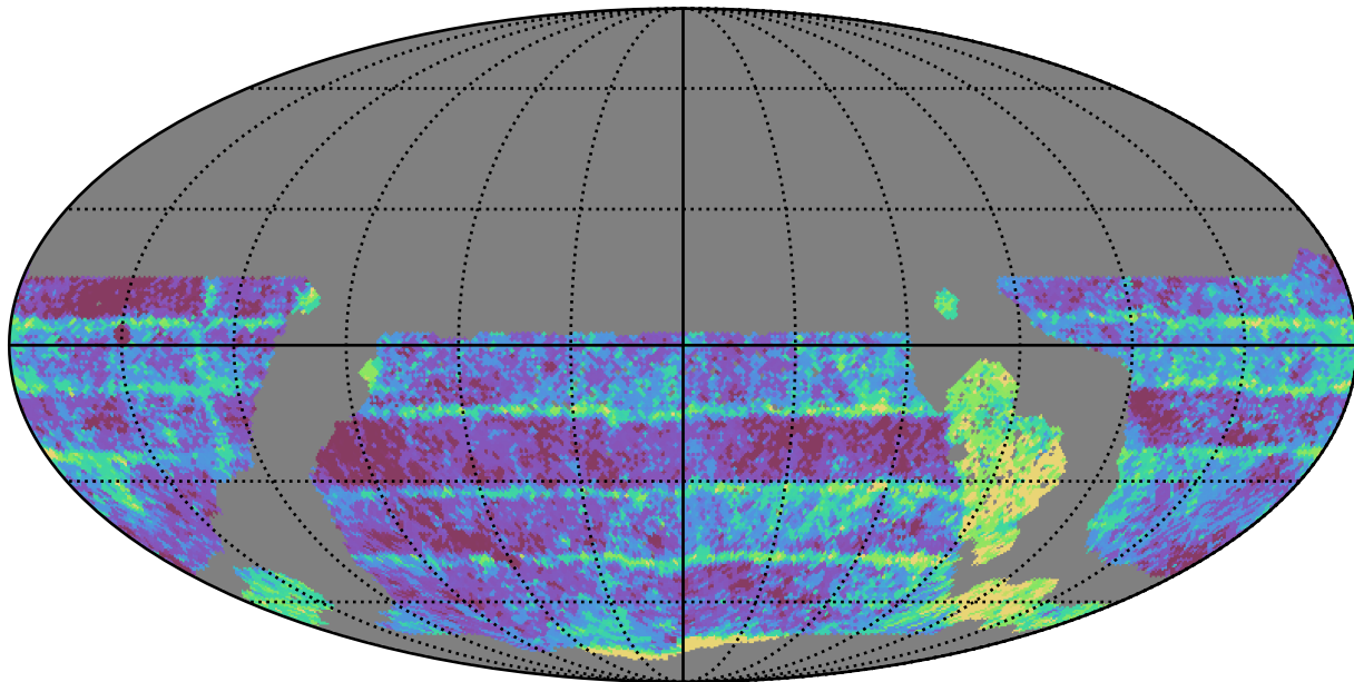
ddf_loaded_fl4_v3.4_10yrs WFD i band: Median Inter-Night Gap
