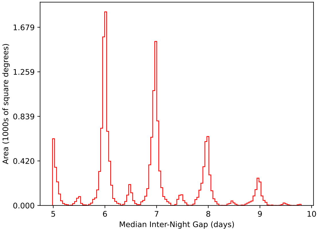
ddf_loaded_fl4_v3.4_10yrs WFD i band: Median Inter-Night Gap
