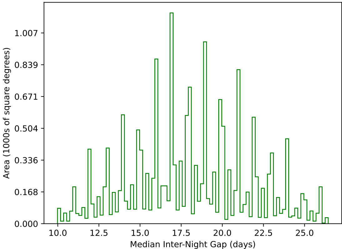
ddf_loaded_fl4_v3.4_10yrs WFD g band: Median Inter-Night Gap
