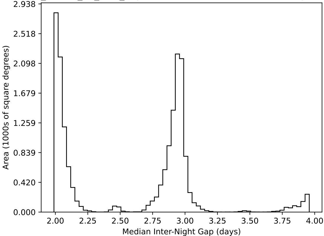
ddf_loaded_fl4_v3.4_10yrs WFD all bands: Median Inter-Night Gap
