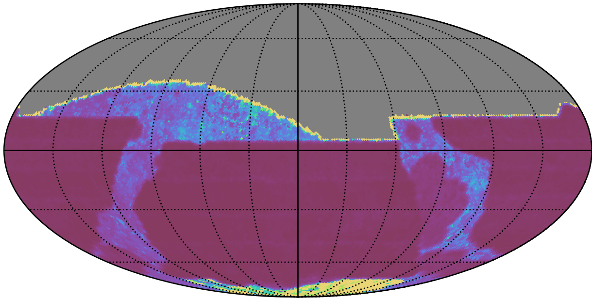
ddf_loaded_fl4_v3.4_10yrs All sky z band: Median Inter-Night Gap
