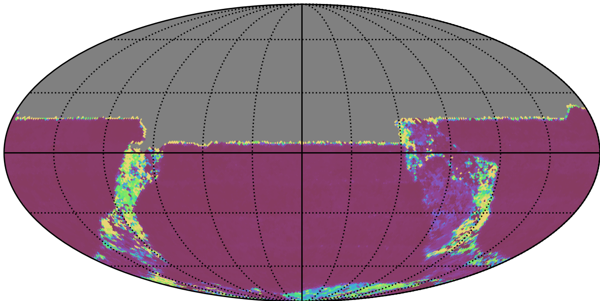
ddf_loaded_fl4_v3.4_10yrs All sky u band: Median Inter-Night Gap
