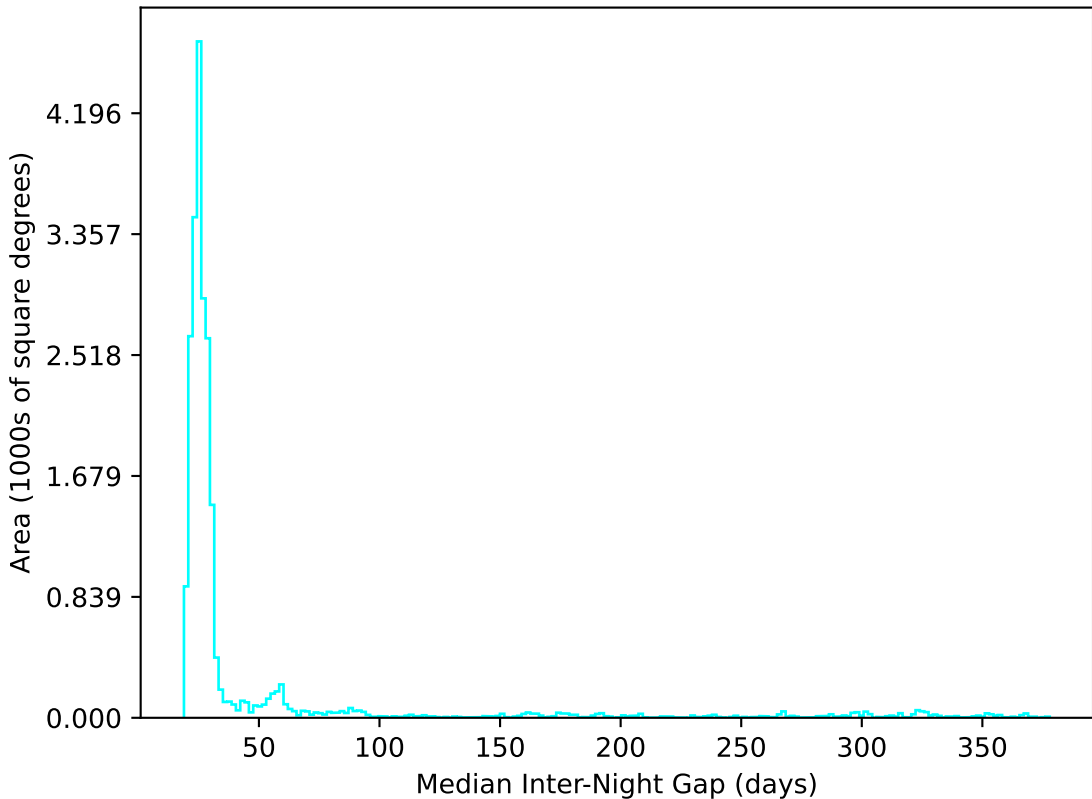
ddf_loaded_fl4_v3.4_10yrs All sky u band: Median Inter-Night Gap
