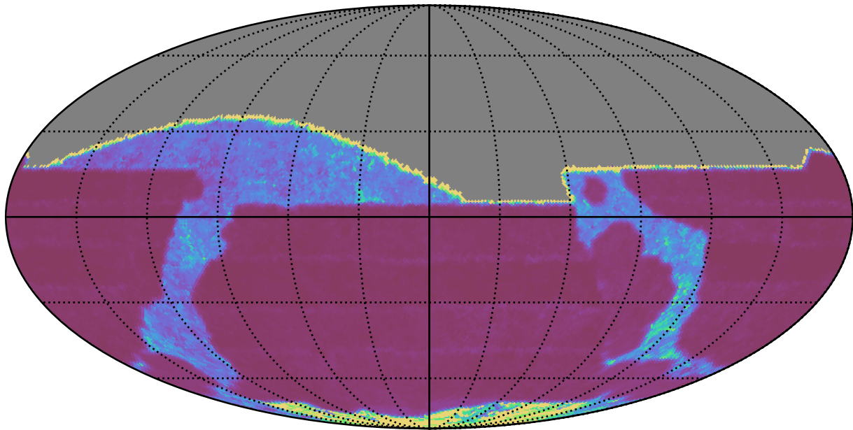
ddf_loaded_fl4_v3.4_10yrs All sky r band: Median Inter-Night Gap
