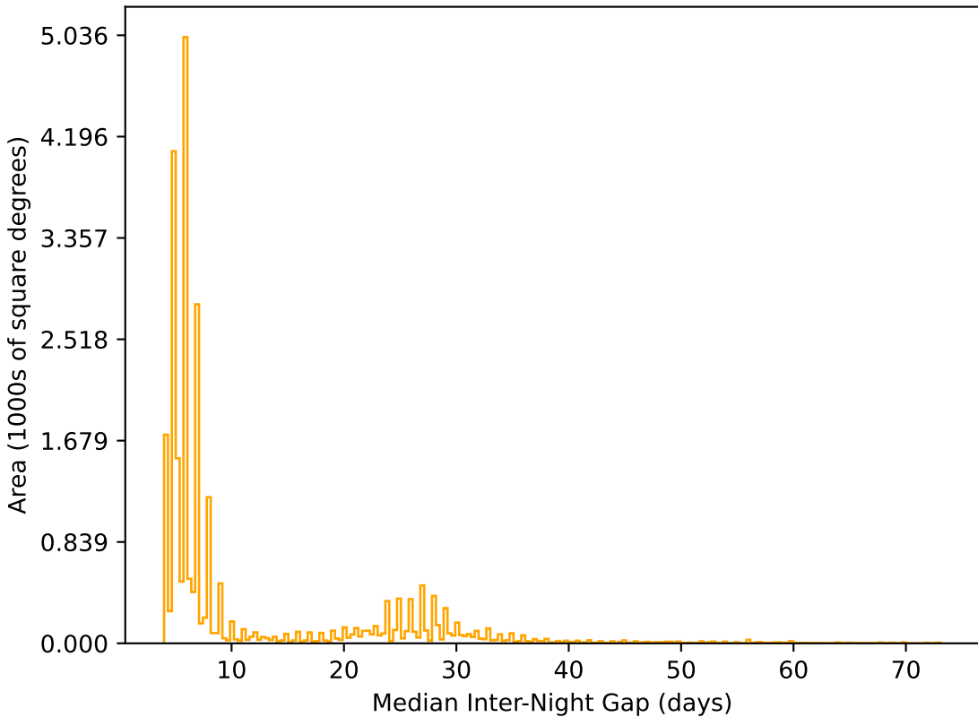
ddf_loaded_fl4_v3.4_10yrs All sky r band: Median Inter-Night Gap
