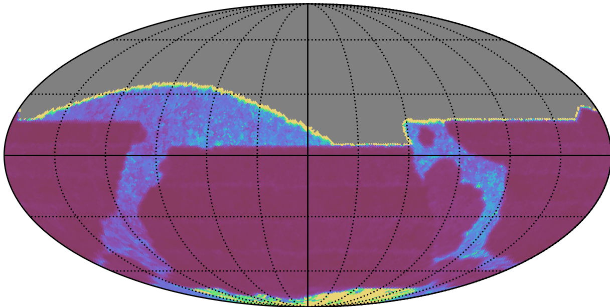
ddf_loaded_fl4_v3.4_10yrs All sky i band: Median Inter-Night Gap
