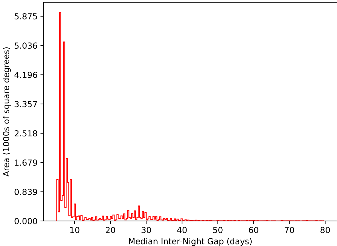
ddf_loaded_fl4_v3.4_10yrs All sky i band: Median Inter-Night Gap
