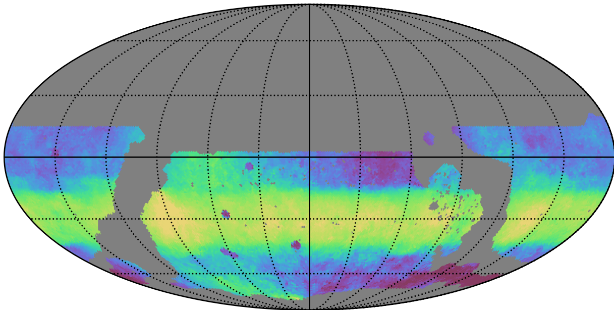
ddf_loaded_fl4_v3.4_10yrs WFD z band: Median HA
