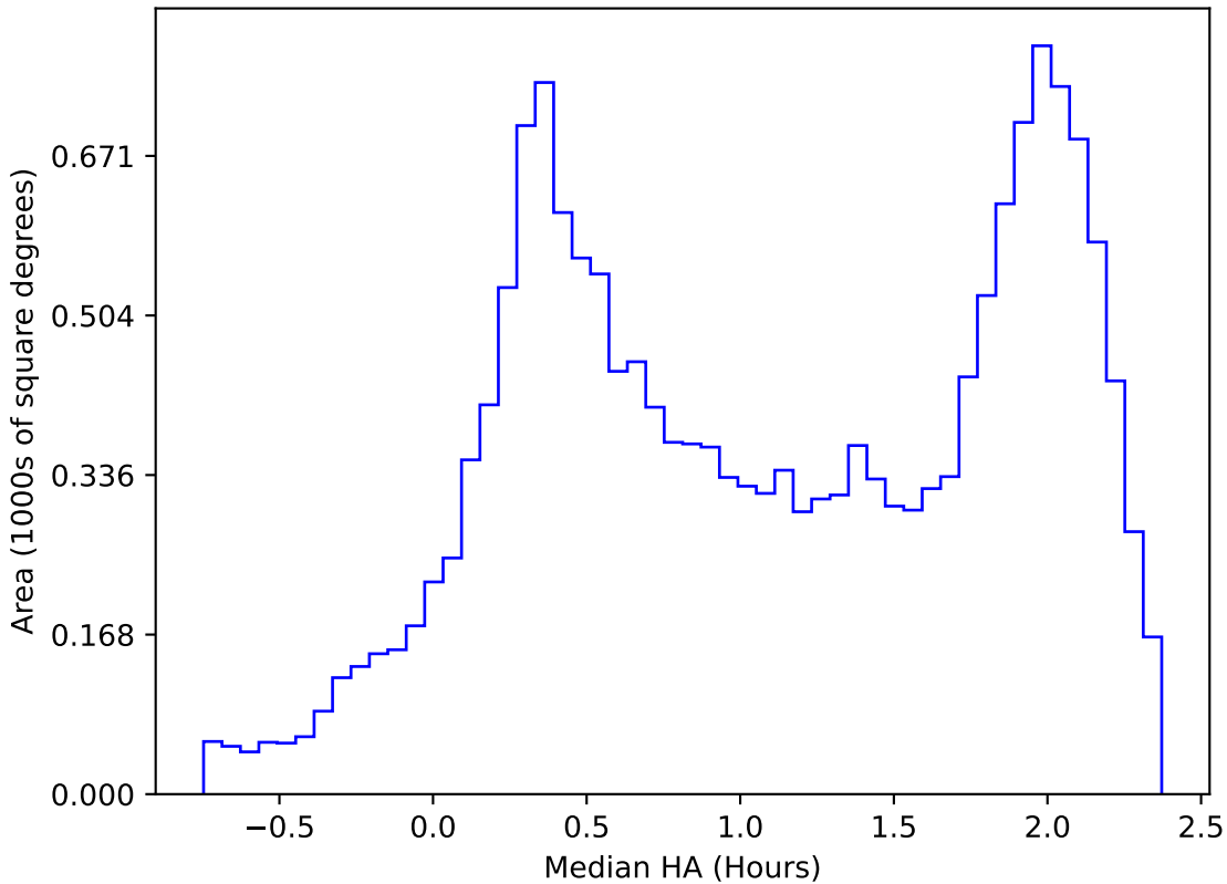
ddf_loaded_fl4_v3.4_10yrs WFD z band: Median HA
