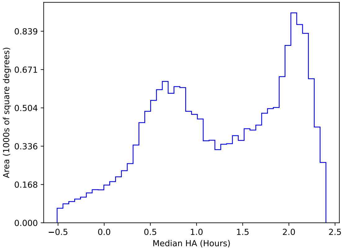
ddf_loaded_fl4_v3.4_10yrs WFD y band: Median HA
