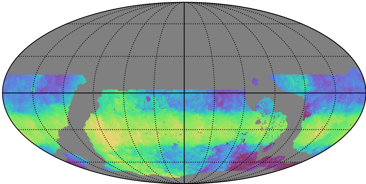
ddf_loaded_fl4_v3.4_10yrs WFD u band: Median HA
