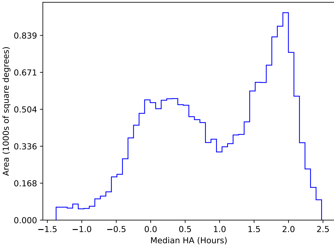
ddf_loaded_fl4_v3.4_10yrs WFD u band: Median HA
