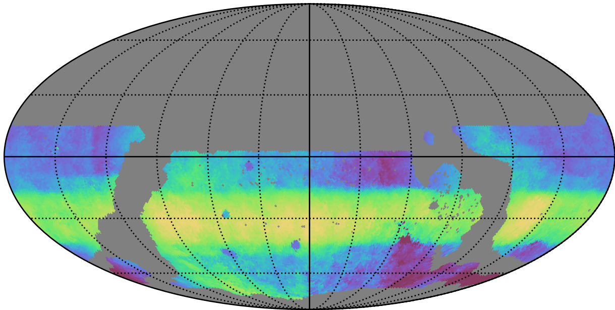
ddf_loaded_fl4_v3.4_10yrs WFD r band: Median HA
