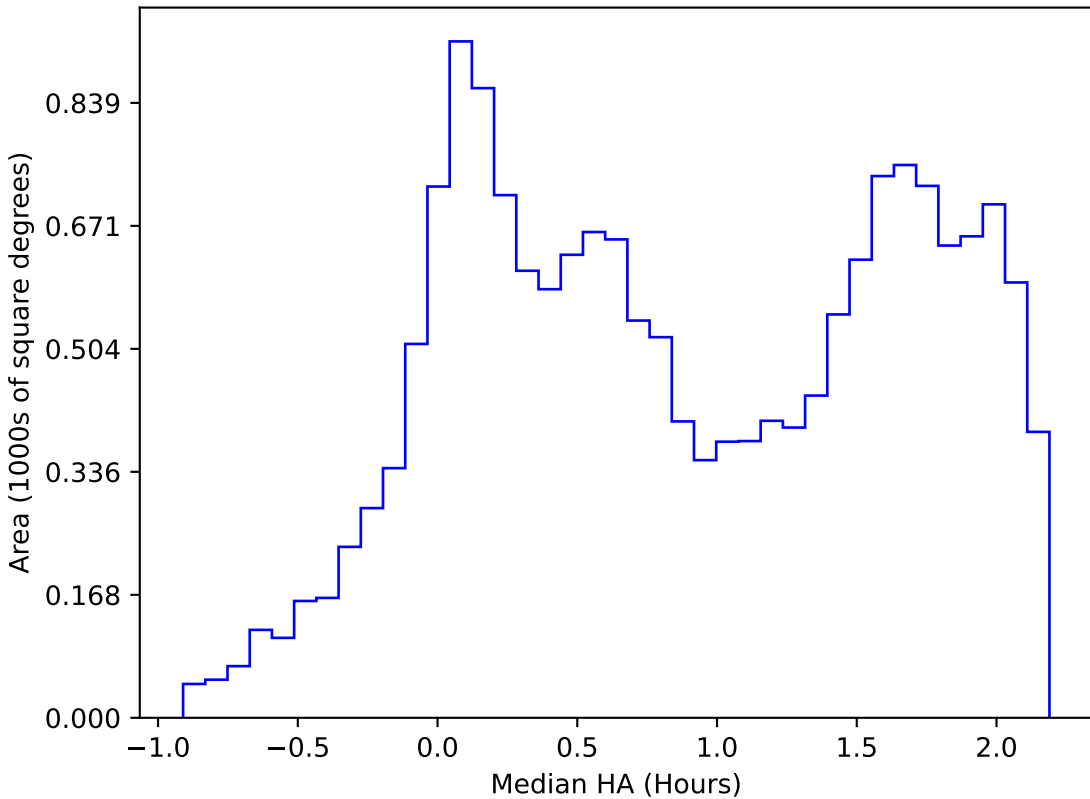
ddf_loaded_fl4_v3.4_10yrs WFD r band: Median HA
