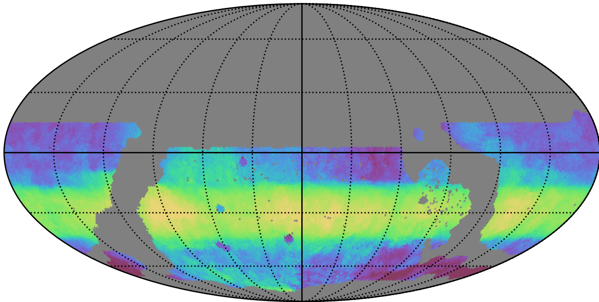
ddf_loaded_fl4_v3.4_10yrs WFD i band: Median HA
