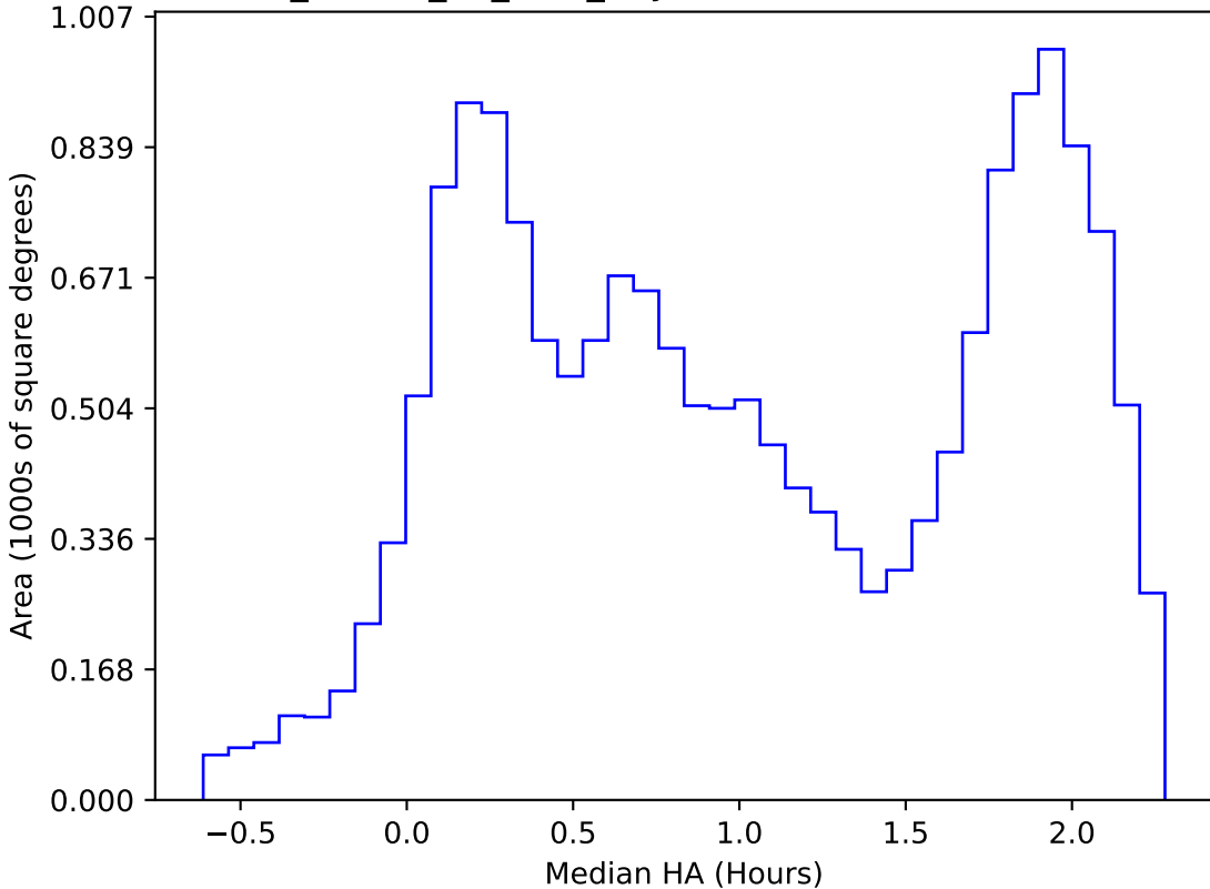
ddf_loaded_fl4_v3.4_10yrs WFD i band: Median HA
