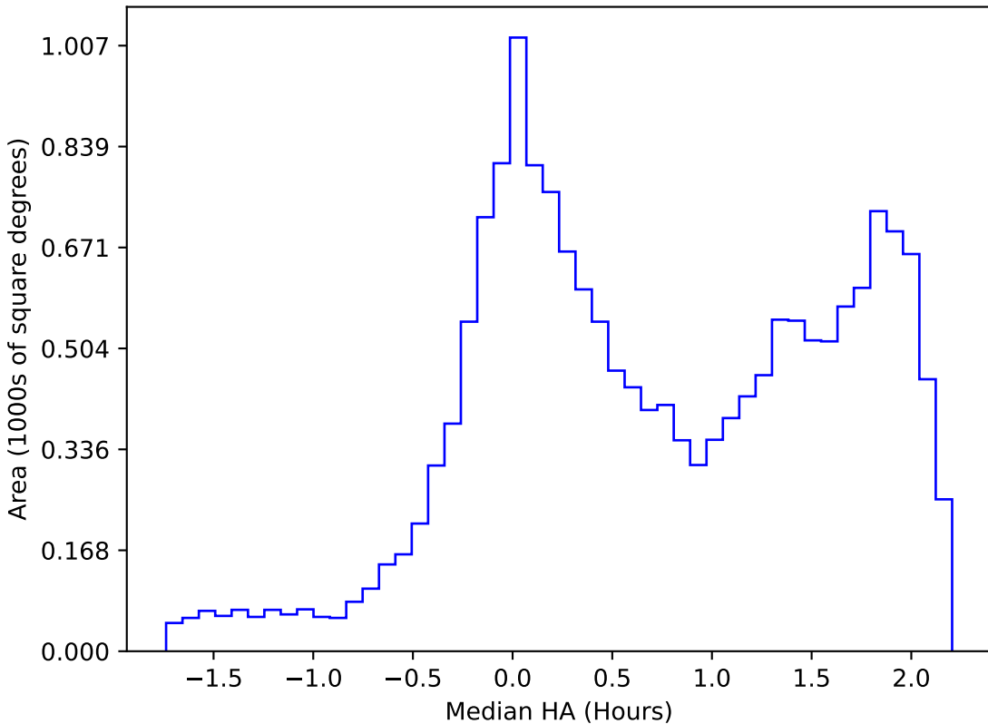
ddf_loaded_fl4_v3.4_10yrs WFD g band: Median HA
