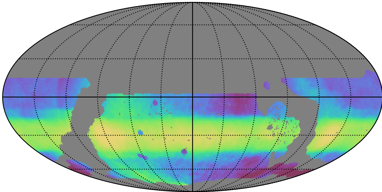
ddf_loaded_fl4_v3.4_10yrs WFD all bands: Median HA
