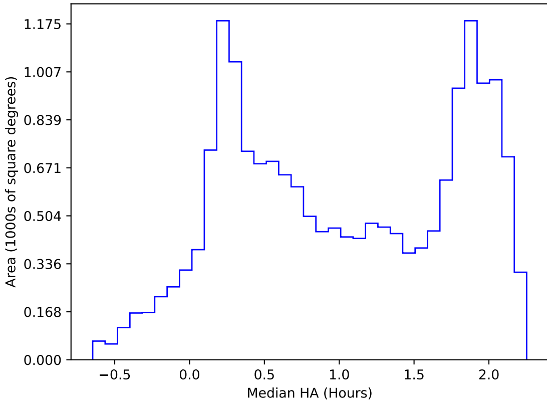
ddf_loaded_fl4_v3.4_10yrs WFD all bands: Median HA
