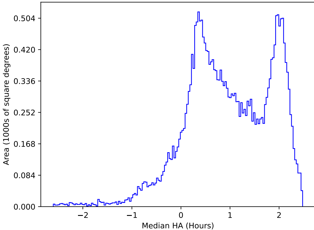
ddf_loaded_fl4_v3.4_10yrs All sky z band: Median HA
