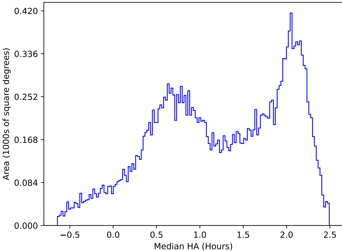
ddf_loaded_fl4_v3.4_10yrs All sky y band: Median HA
