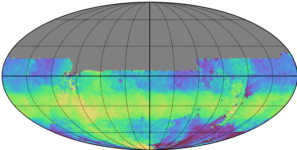
ddf_loaded_fl4_v3.4_10yrs All sky u band: Median HA
