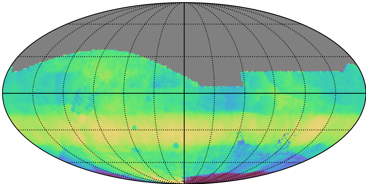
ddf_loaded_fl4_v3.4_10yrs All sky r band: Median HA
