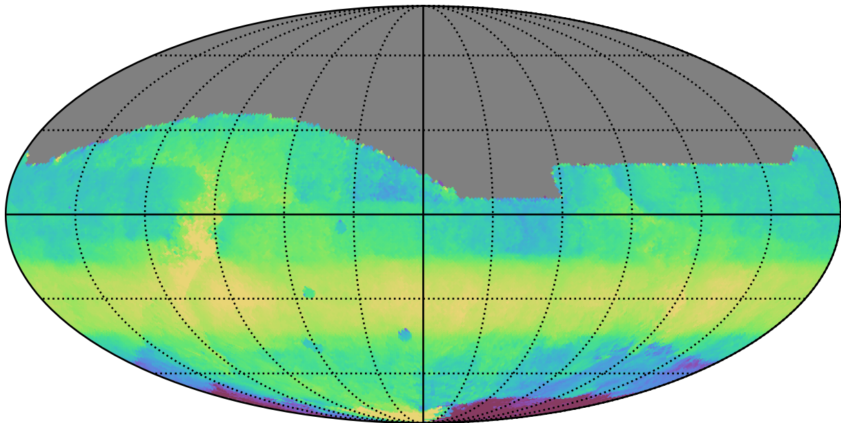
ddf_loaded_fl4_v3.4_10yrs All sky i band: Median HA
