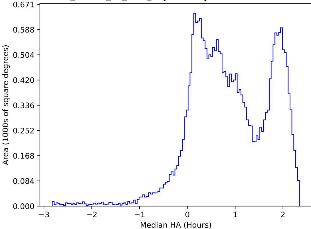
ddf_loaded_fl4_v3.4_10yrs All sky i band: Median HA
