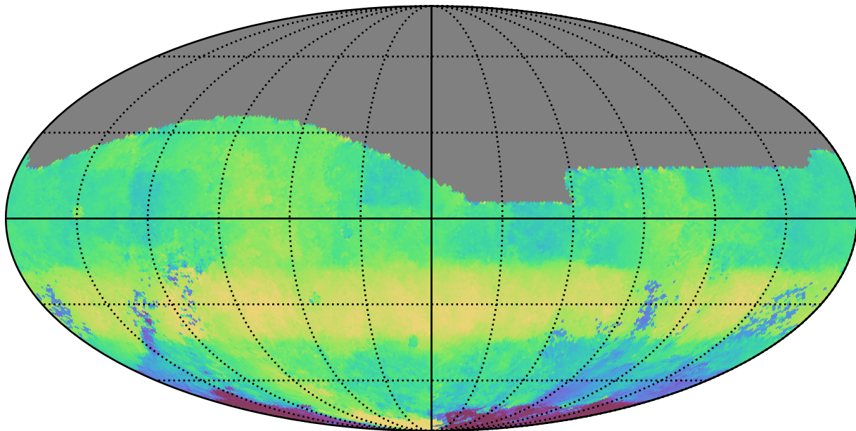
ddf_loaded_fl4_v3.4_10yrs All sky g band: Median HA
