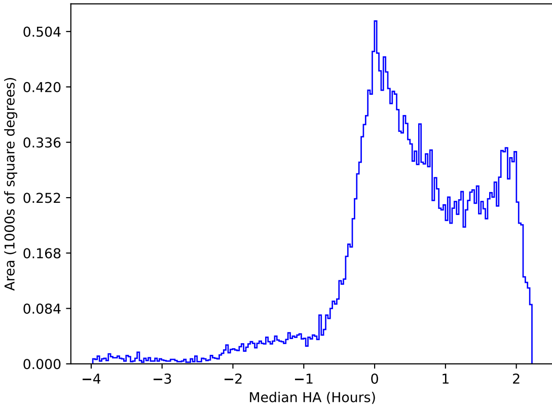
ddf_loaded_fl4_v3.4_10yrs All sky g band: Median HA
