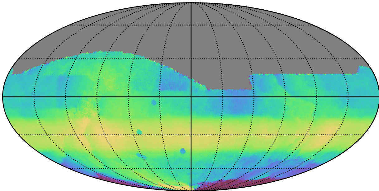
ddf_loaded_fl4_v3.4_10yrs All sky all bands: Median HA
