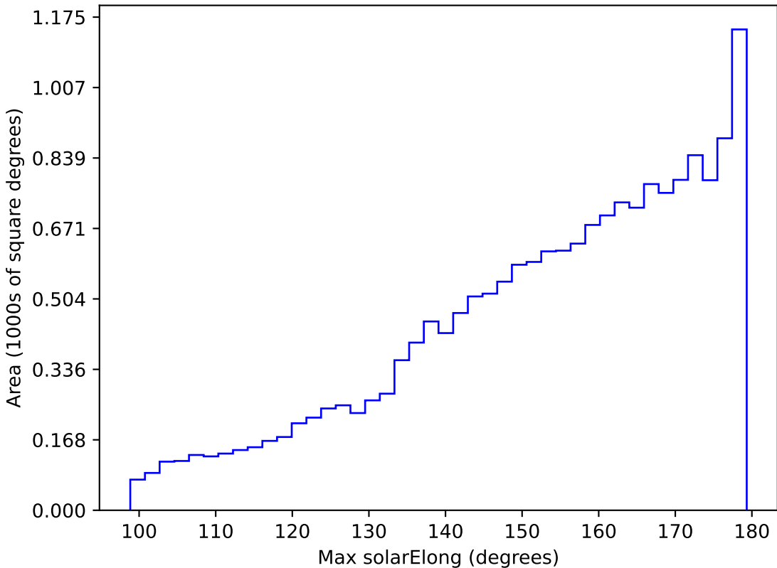
ddf_loaded_fl4_v3.4_10yrs WFD z band: Max solarElong
