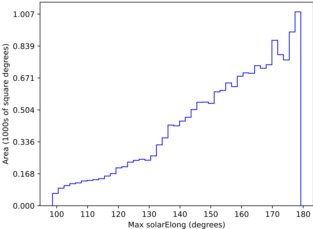
ddf_loaded_fl4_v3.4_10yrs WFD y band: Max solarElong
