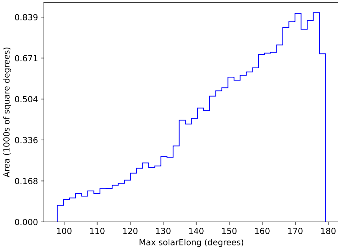
ddf_loaded_fl4_v3.4_10yrs WFD u band: Max solarElong
