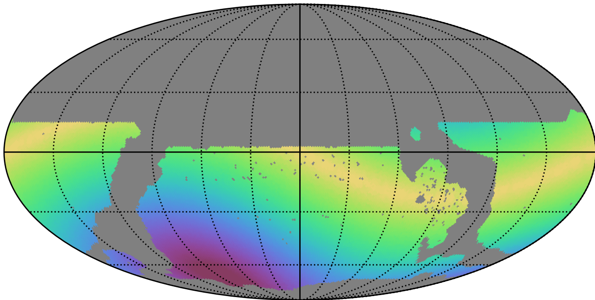
ddf_loaded_fl4_v3.4_10yrs WFD r band: Max solarElong
