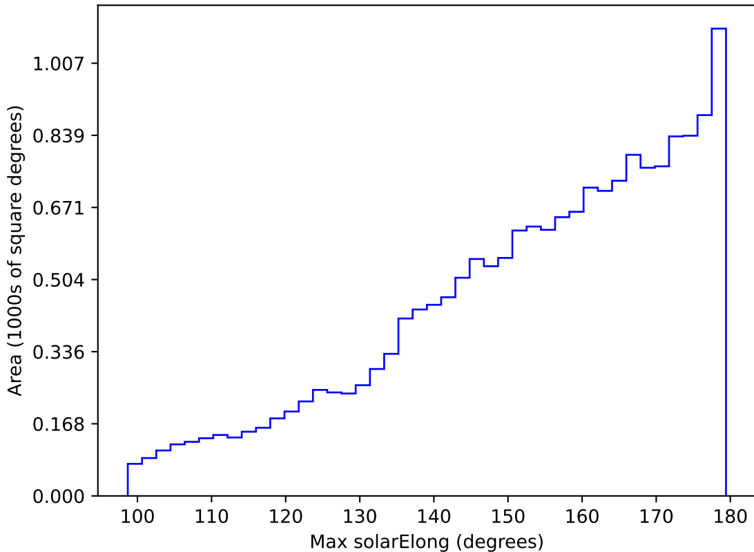
ddf_loaded_fl4_v3.4_10yrs WFD r band: Max solarElong
