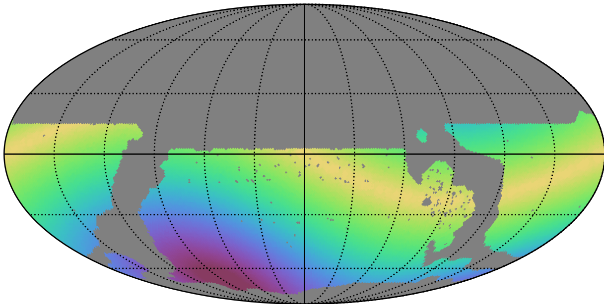
ddf_loaded_fl4_v3.4_10yrs WFD i band: Max solarElong
