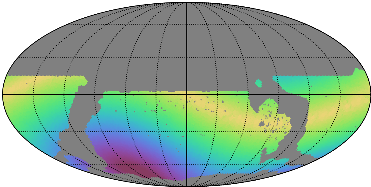
ddf_loaded_fl4_v3.4_10yrs WFD g band: Max solarElong
